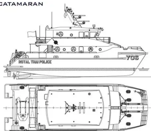
23м. CATAMARAN
